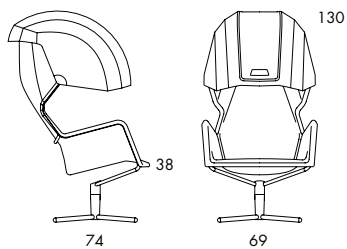
O43H 12.6 kg | 0.85 m 3 /pc (1.45 m 3 /2 pcs)
